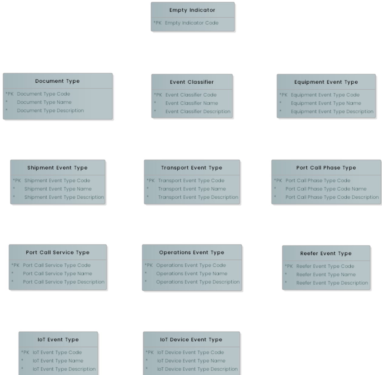
Figure 23: Events reference data entities
