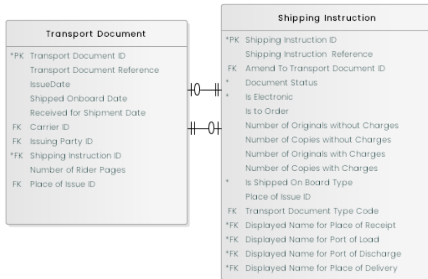
Figure 10: Transport Document subject area
