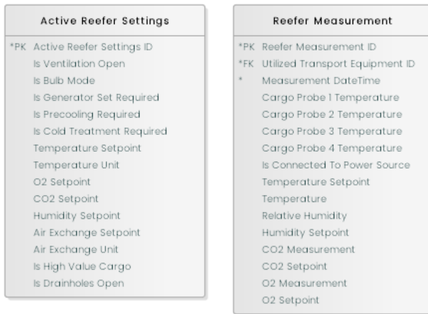
Figure 27: Reefer subject area
