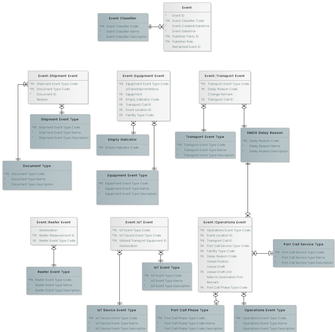
Figure 22: Events subject area
