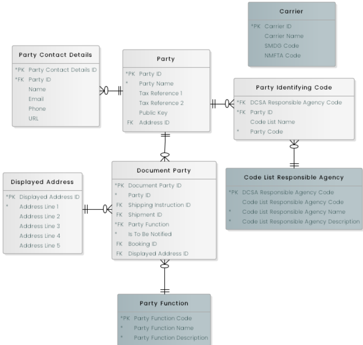
Figure 11: Party subject area
