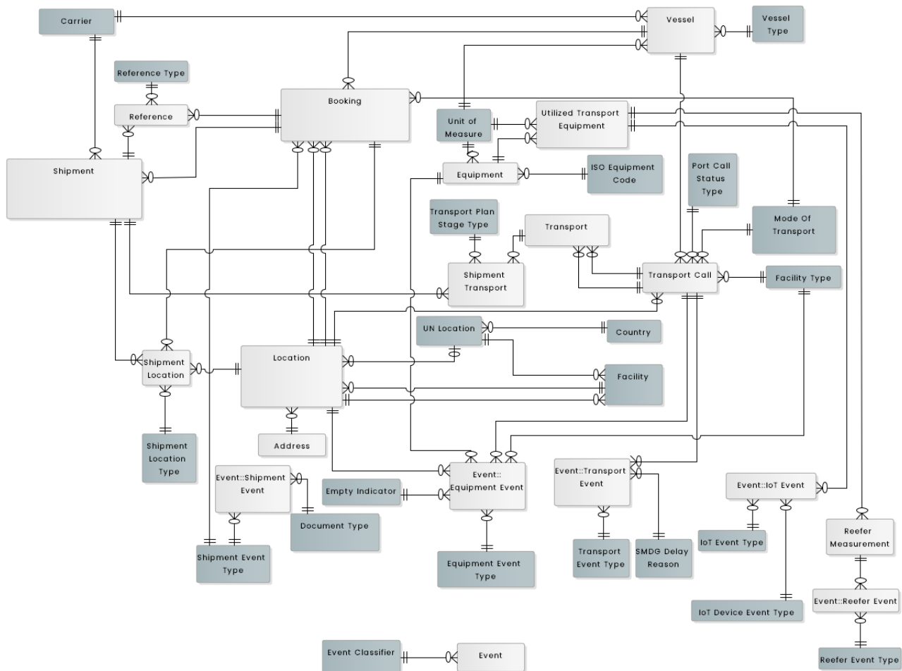
Figure 4: Logical Data Model for track and trace
