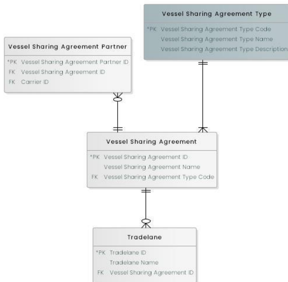
Figure 24: VSA subject area
