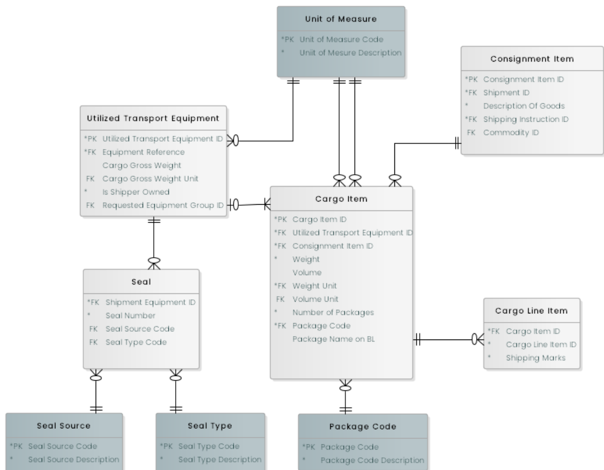
Figure 16: Stuffing subject area
