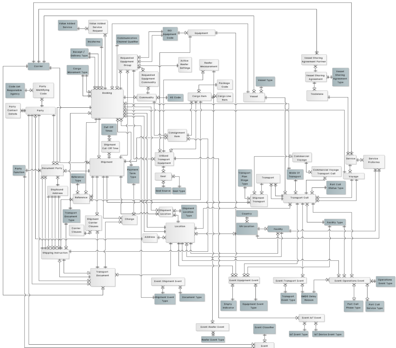
Figure 3: Logical Data Model - overview of data entities
