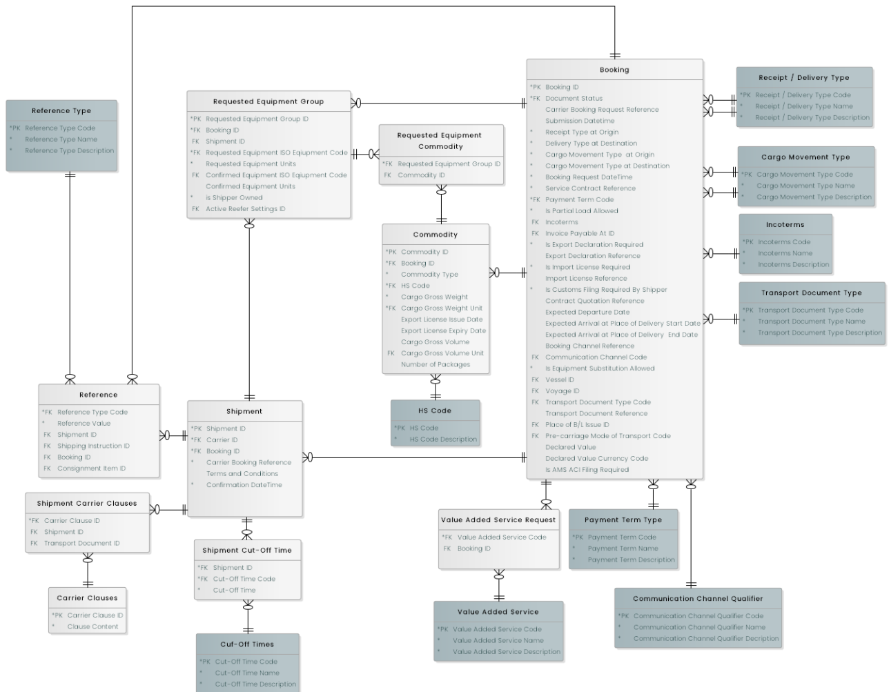
Figure 8: Shipment subject area
