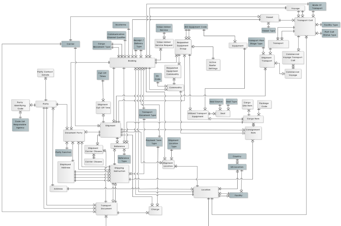
Figure 6: Logical Data Model for eDocumentation
