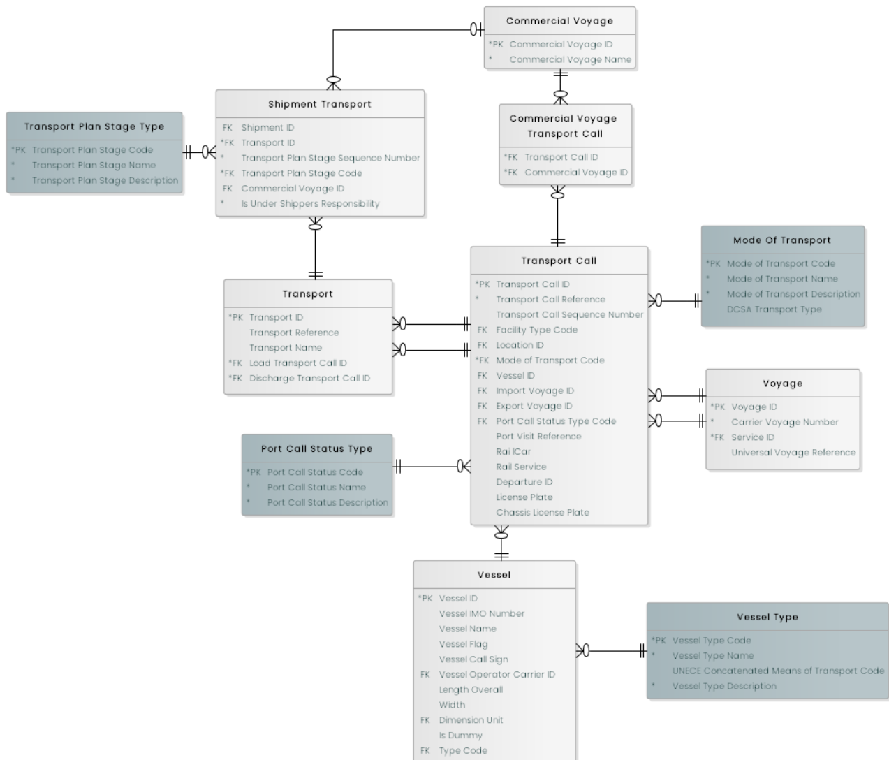
Figure 20: Transport subject area
