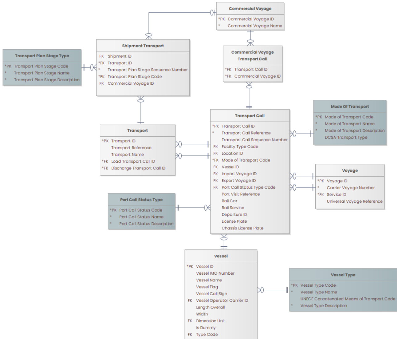
Figure 19: Transport subject area
