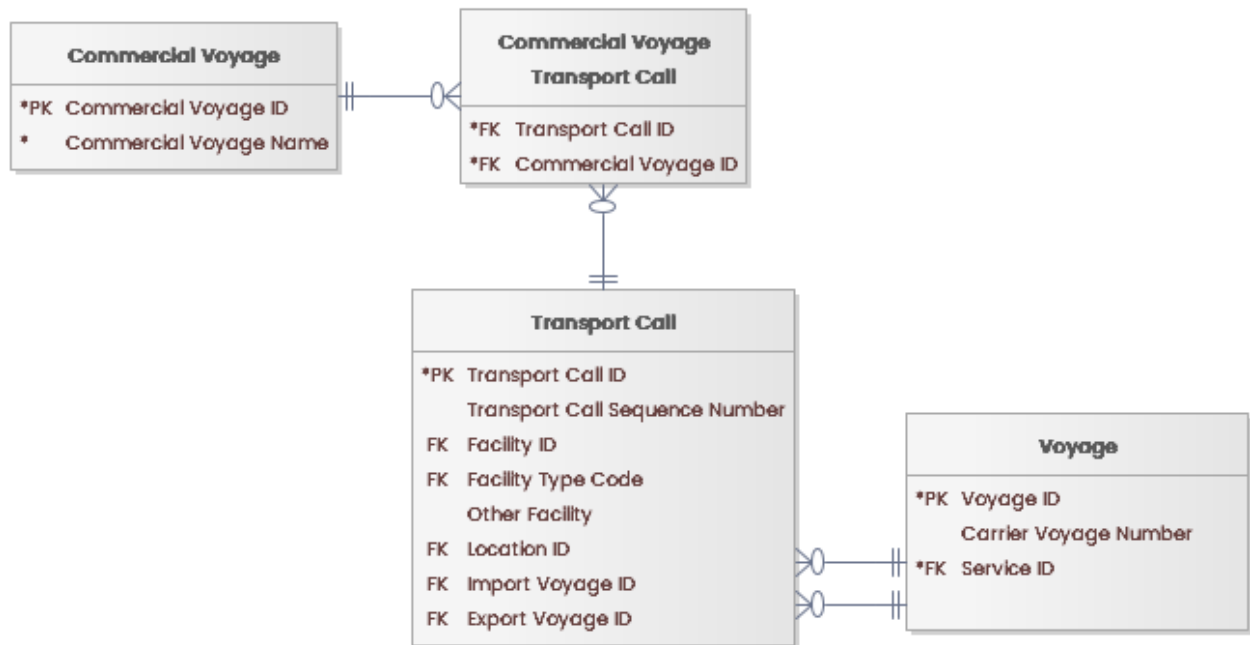
Figure 28: Transport Journey subject area
