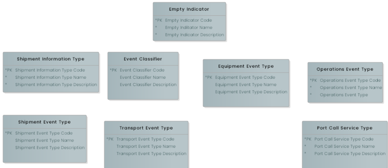
Figure 24: Events reference data entities
