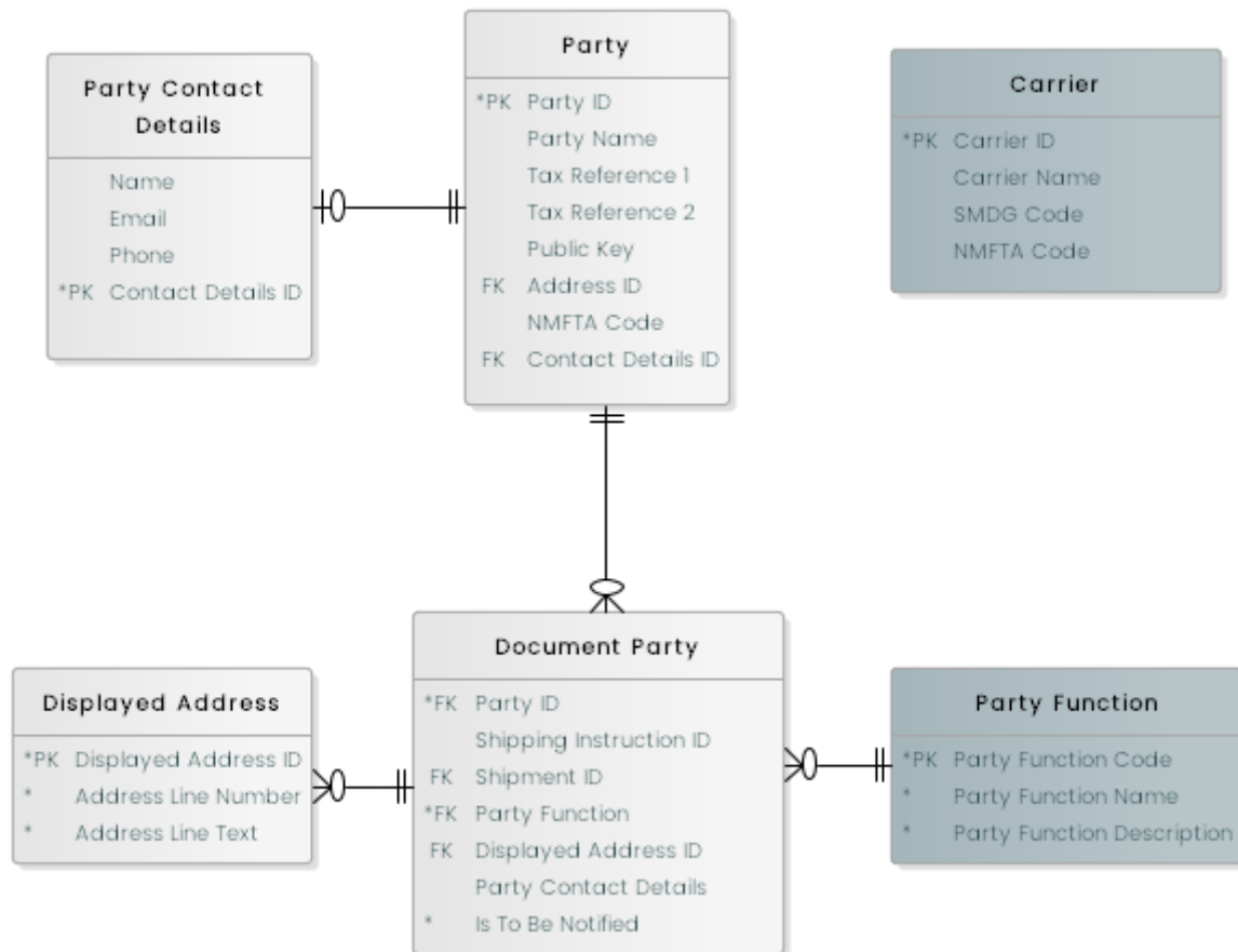
Figure 12: Party subject area
