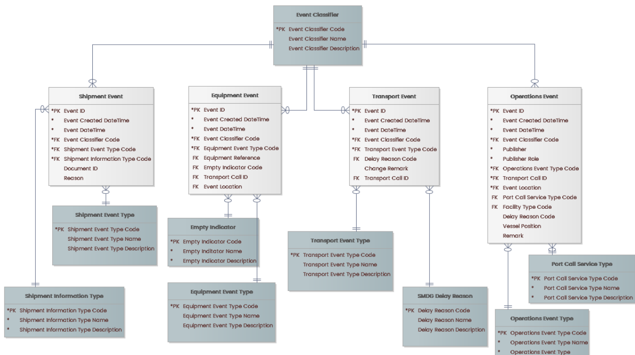
Figure 23: Events subject area
