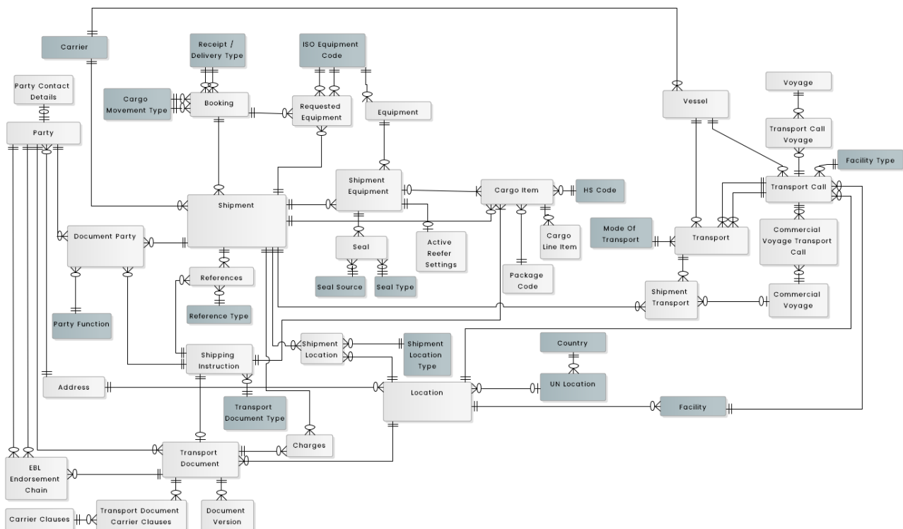
Figure 6: Logical Data Model for eDocumentation
