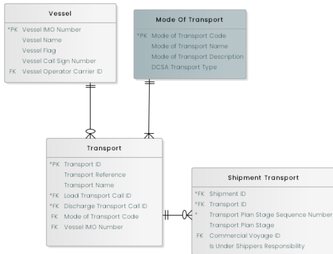
Figure 21: Transport subject area
