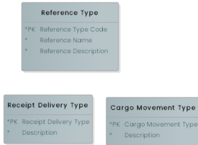
Figure 9: Shipment reference data entities
