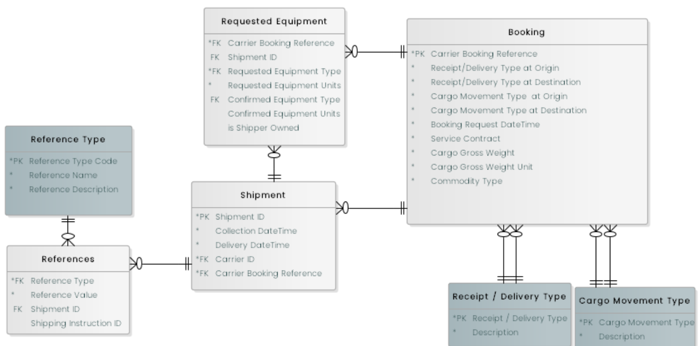
Figure 8: Shipment subject area
