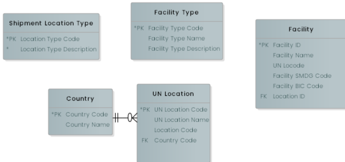
Figure 20: Location reference data entities
