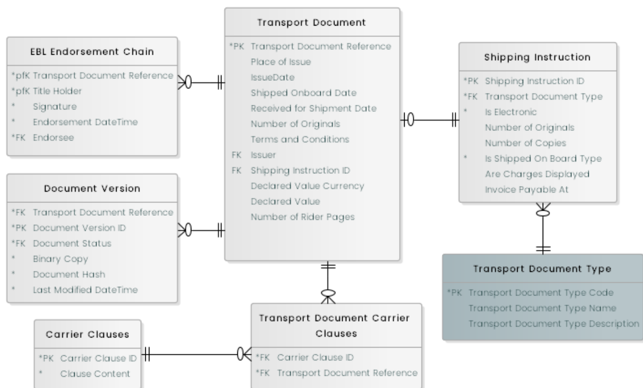
Figure 10: Transport Document subject area
