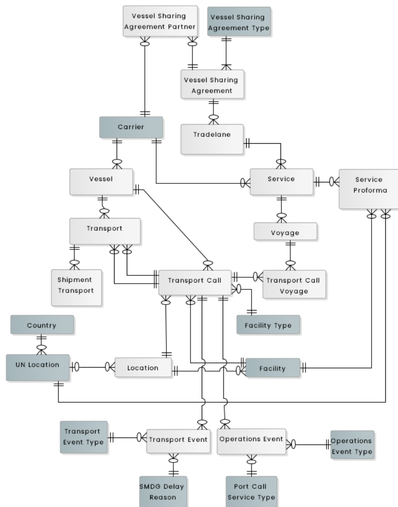
Figure 5: Logical Data Model for operational vessel schedules
