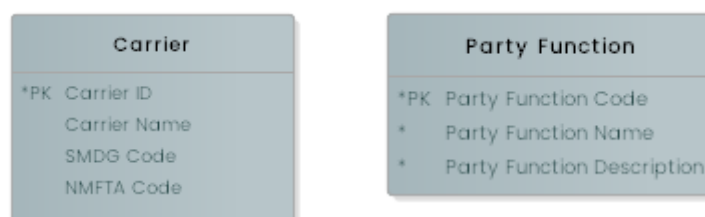
Figure 13: Party reference data entities
