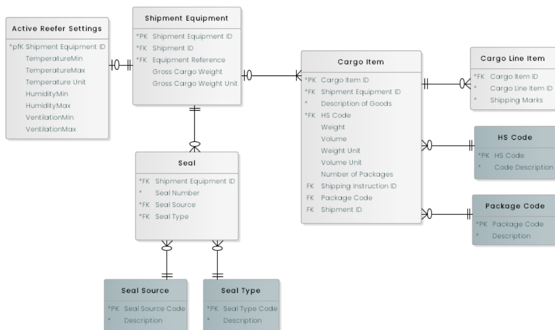
Figure 17: Stuffing subject area
