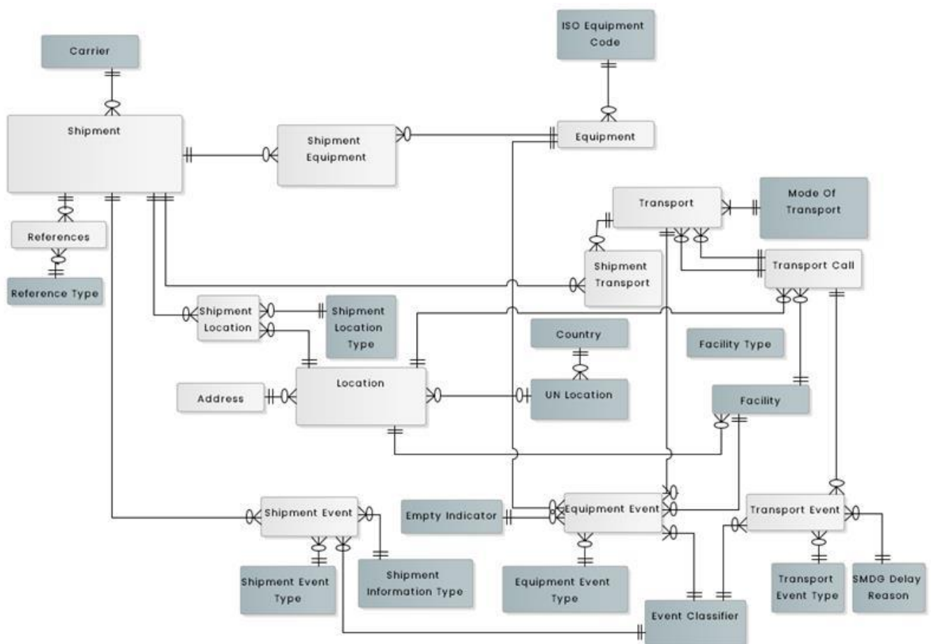
Figure 4: Logical Data Model for track and trace
