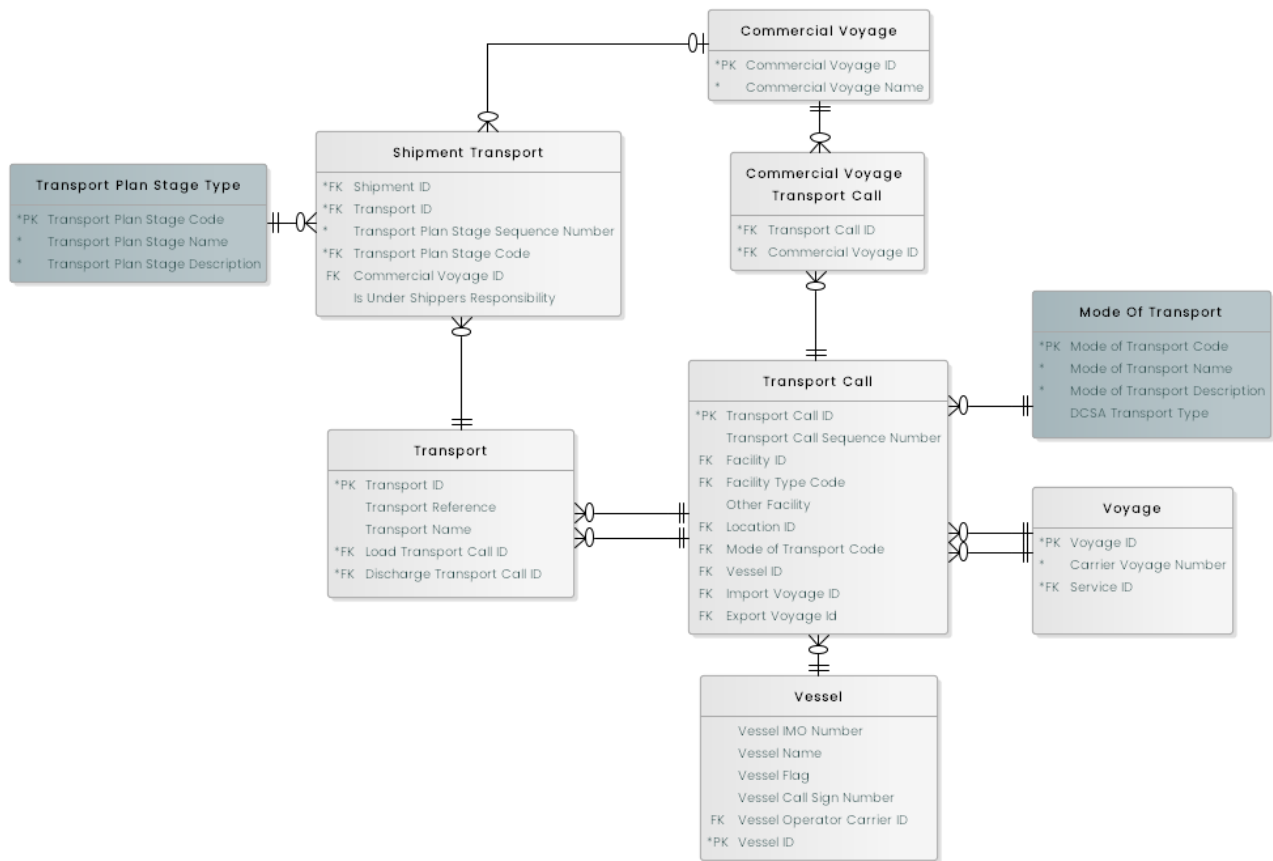
Figure 21: Transport (Journey) subject area
