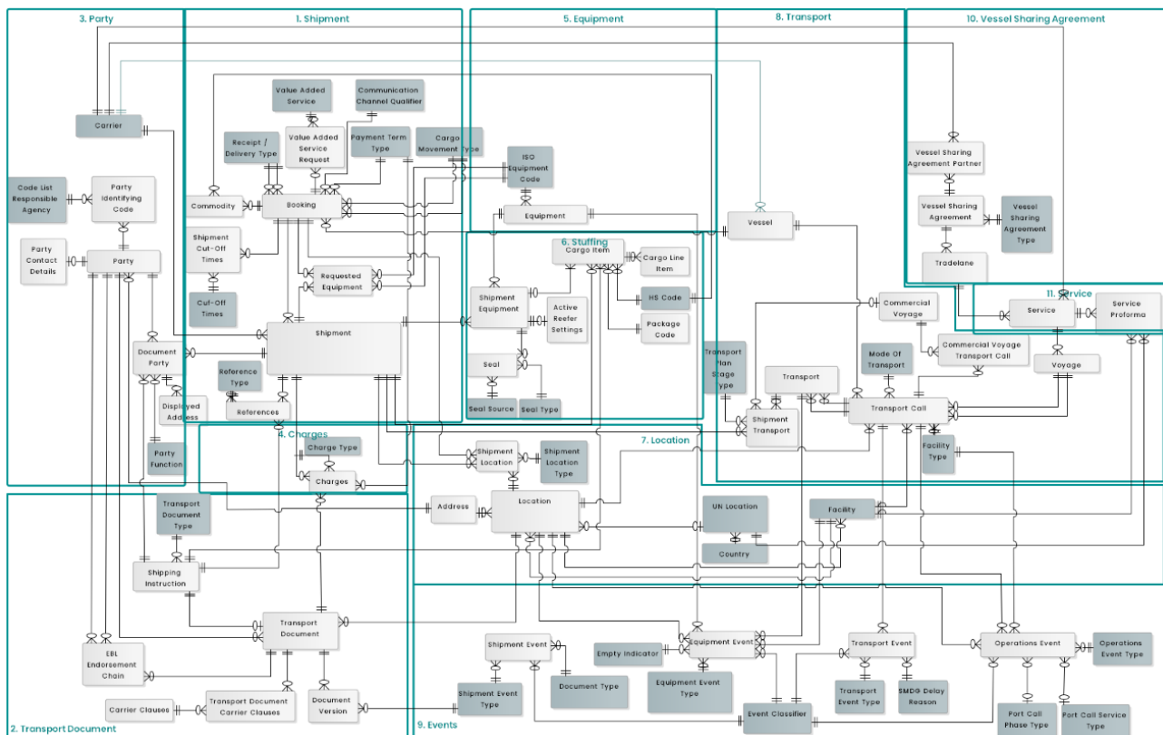
Figure 7: Subject areas in the Logical Data Model
